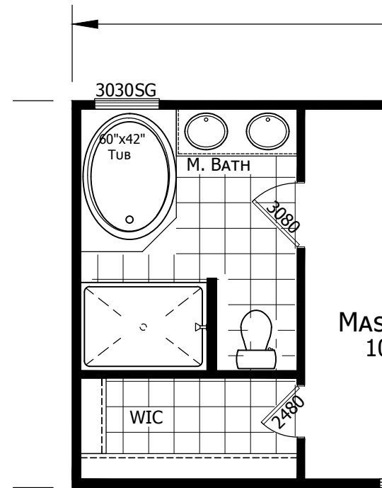
OPTIONAL M. BATH w/ 42" DECK TUB
